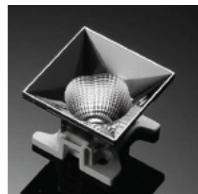
AE-030A-FW Beam Angle: Flood 60°
